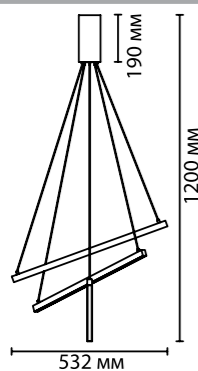
3860/39L 1 × LED × 39W, 2180 lm крепёж: планка
