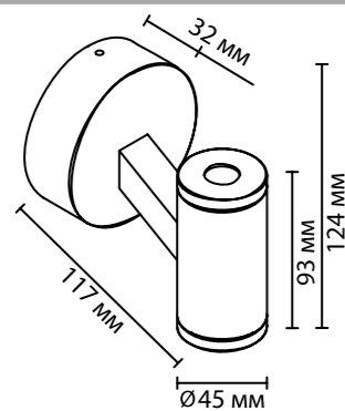
6636/6BL, 6636/6WL 1×LED × 6W, 540 lm крепеж: планка
