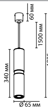
4742/5L 1 x GU10 LED x 5W крепёж: планка
