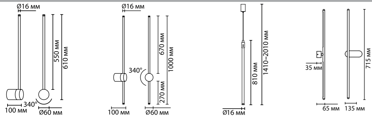
4335/12WL, 4335/12WG 1 × LED × 12W, 675 lm крепёж: планка
