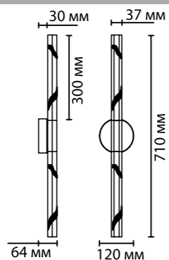
6679/6WL 1 × LED × 6W, 360 lm крепёж: планка
