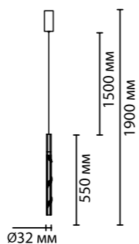
6679/4L 1 × LED × 4W, 240 lm крепёж: планка
