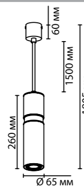
4743/5L, 4744/5L, 4745/5L 1 x GU10 LED x 5W крепёж: планка
