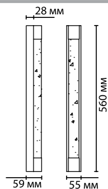
6680/12WL, 6681/12WL 1 × LED × 12W, 600 lm крепёж: планка
